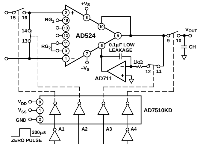
Figure 45. Autozero Circuit
