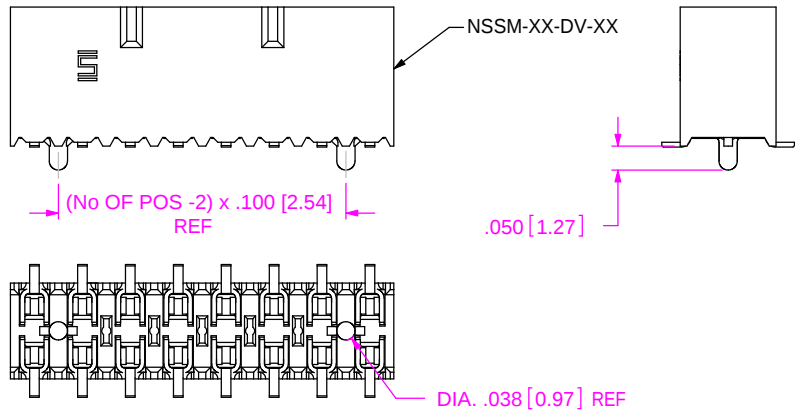
FIGURE 3 -A: ALIGNMENT PIN MOLDED (4 POSITION MIN)
