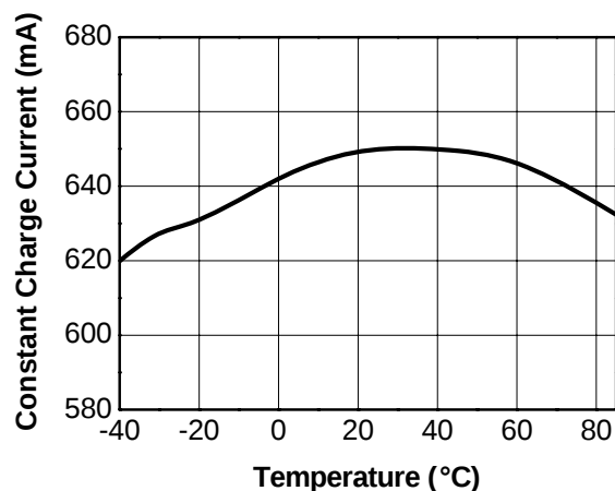
Figure 11. Constant Charge Current vs Temperature I_{CHG} = 650 mA, V_{IN} = 5.0 V, V_{BAT} = 3.9 V
