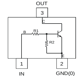
Schematic and Pin Configuration
