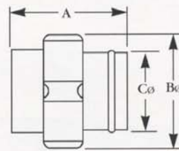
Inline Plug
