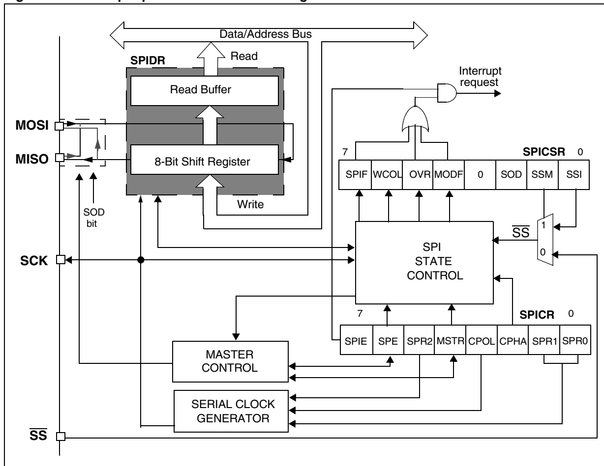
Figure 73. Serial peripheral interface block diagram
