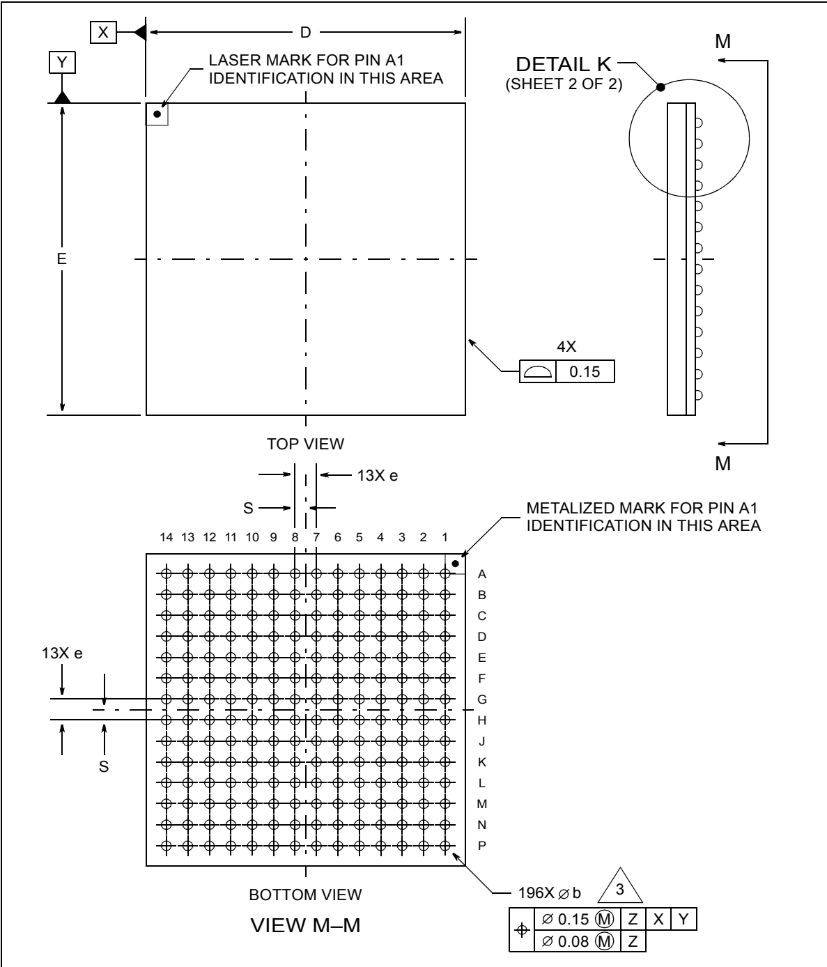
Figure 8-1. 196 MAPBGA Nomenclature
