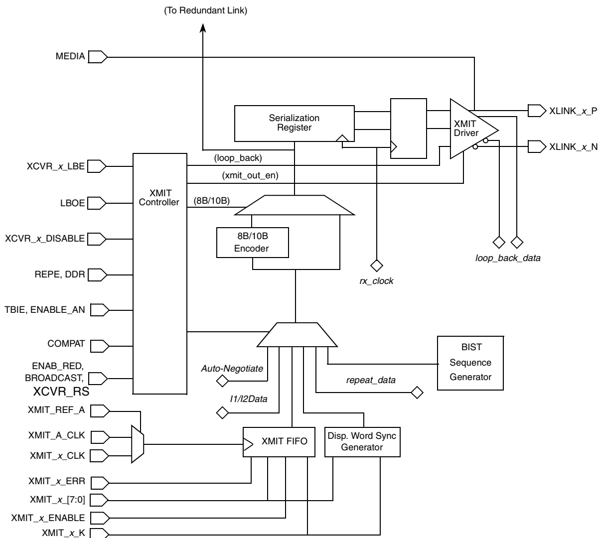
Figure 2-1. MC92604 Transmitter Block Diagram
