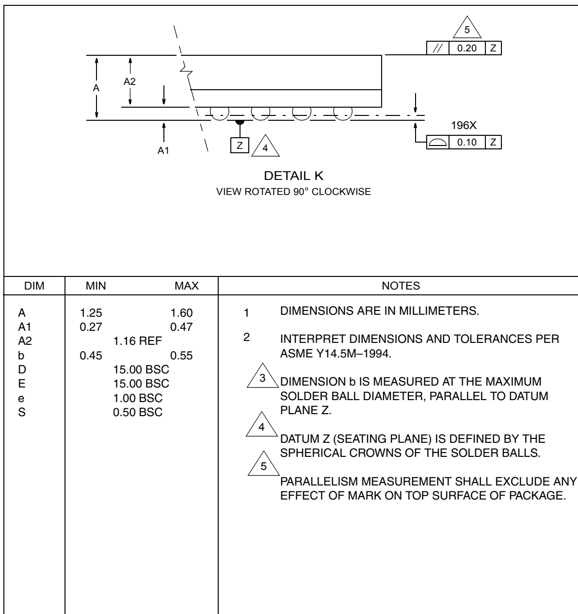
Figure 8-2. 196 MAPBGA Dimensions
