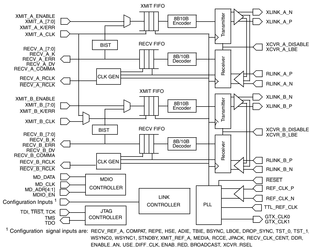
Figure 1-2. MC92604 Block Diagram
