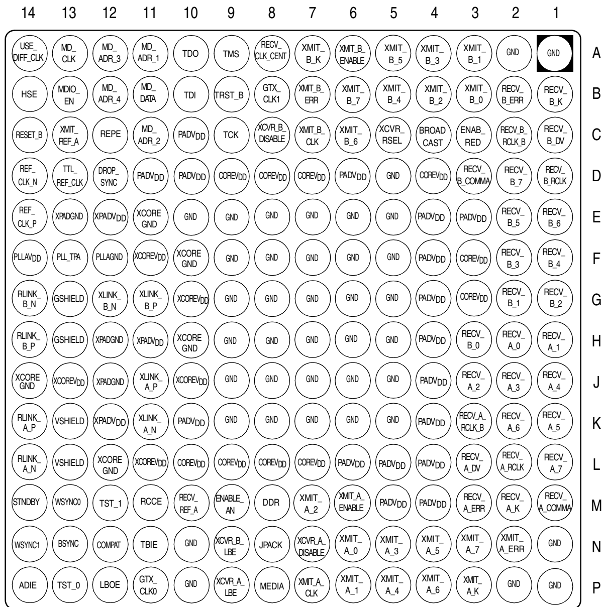
Figure 8-3. MC92604 Package Ball Mapping
