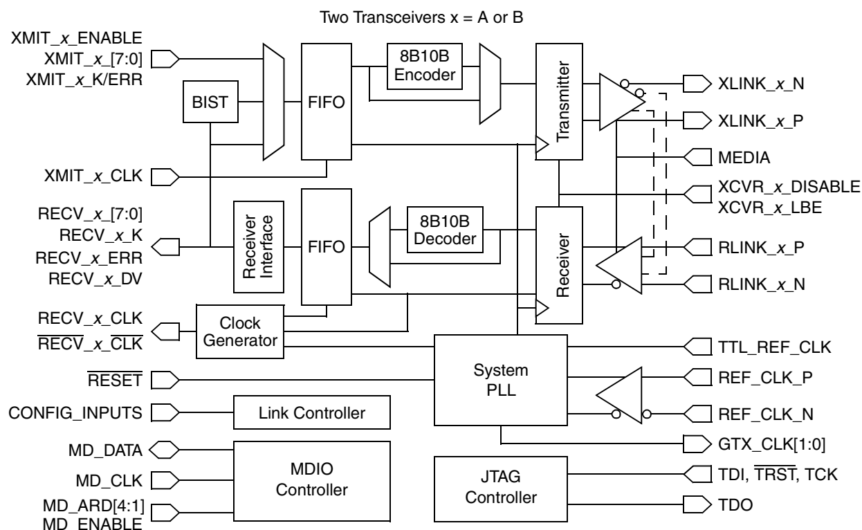
Figure 1-1. MC92604 Simplified Block Diagram
