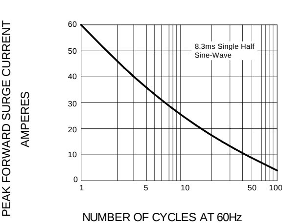
FIG.4 --REPE FORWARD SURGE CURRENT
