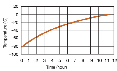
Pull-up characteristics during power failure
