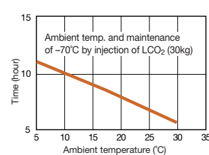
CO 2 backup system operation characteristics
