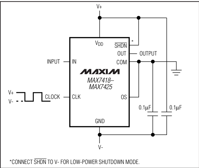
Figure 5. Dual-Supply Operation
