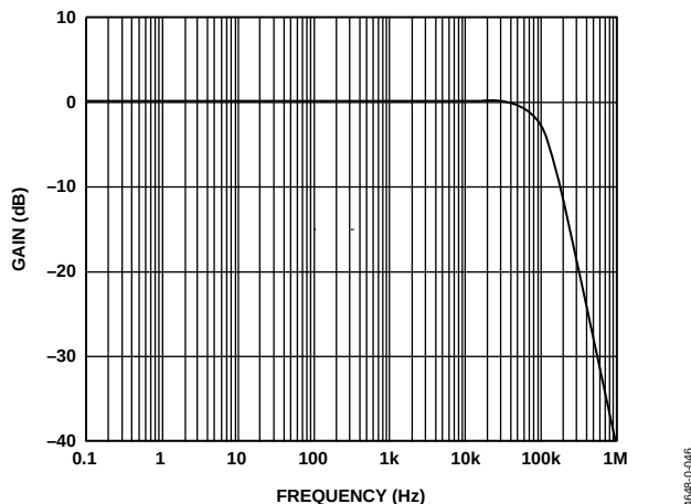
Figure 48. Second-Order Butterworth Low-Pass Filter Frequency Response
