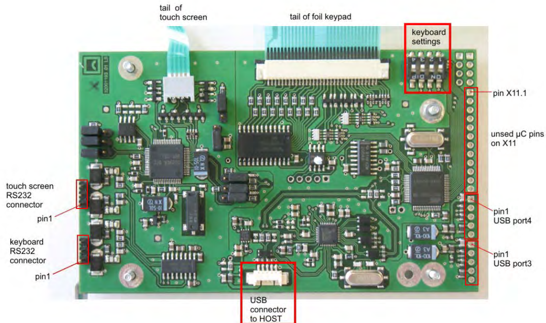
Figure 1 - Keyboard interface
