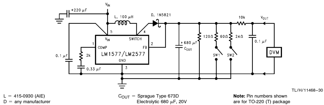
FIGURE 1. Circuit Used to Specify System Parameters for 12V Versions
