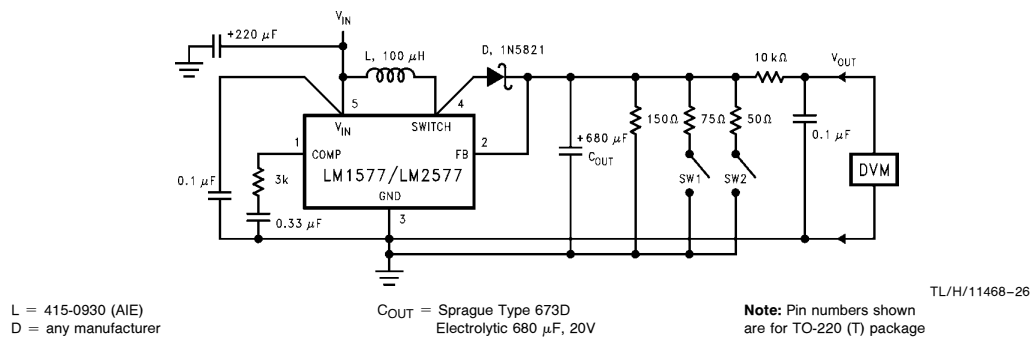
FIGURE 2. Circuit Used to Specify System Parameters for 15V Versions
