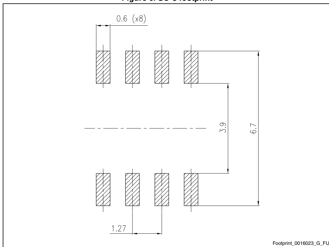
Figure 6. SO-8 footprint
