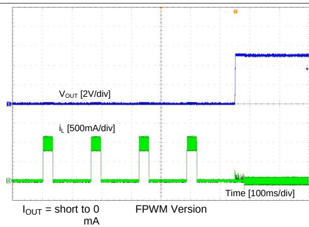
Figure 26. Short Recovery
