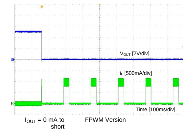
Figure 25. Short Protection
