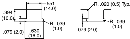
Thru Hole Panel Cut-Out
