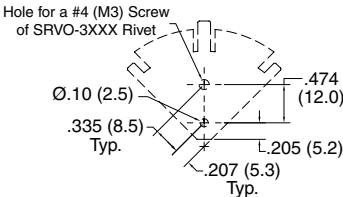
Recommended Mounting Holes
