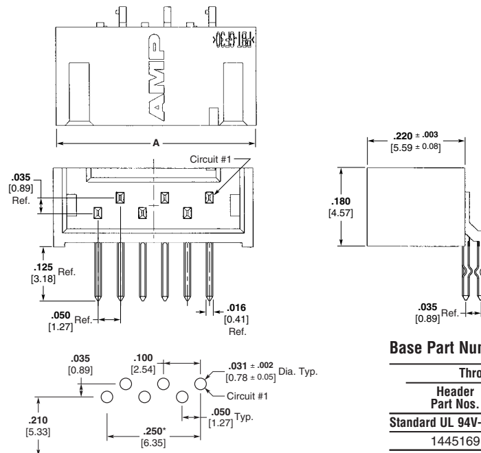
Recommended Mounting Hole Size and Pattern for .062 [1.57] Thick PC Board
