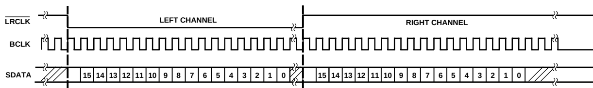
Figure 10. Serial Interface I 2 S-Justified Mode
