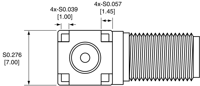
BOTTOM VIEW
