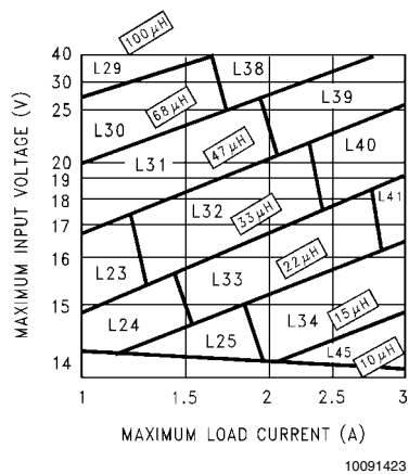
FIGURE 5. LM2676-12
