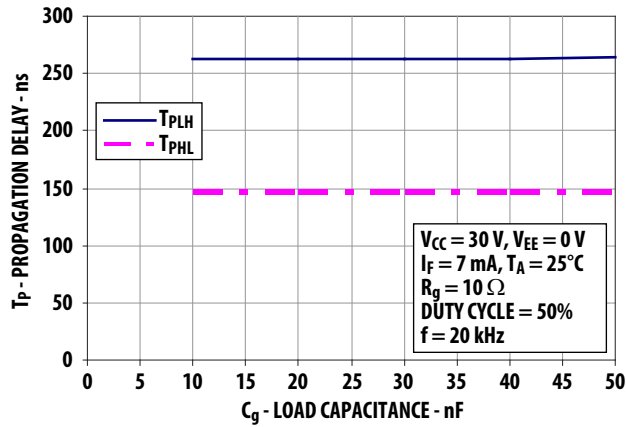
Figure 21. Propagation delay vs. C_g .
