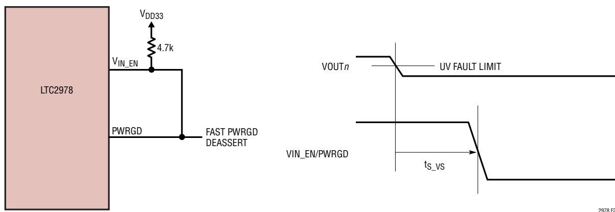
Figure 22. PWRGD Deassert
