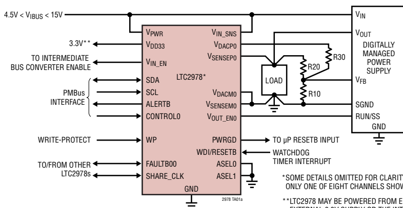
Octal Power Supply Controller with PMBus Interface
