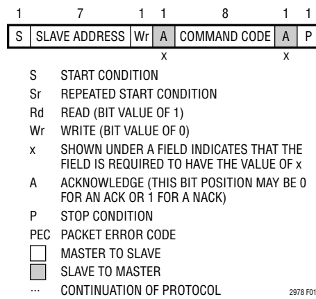
Figure 1a. PMBus Packet Protocol Diagram Element Key
