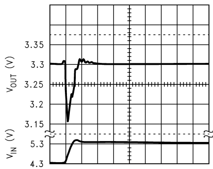
Line Transient Response ( I_{OUT} = 3.0A )
