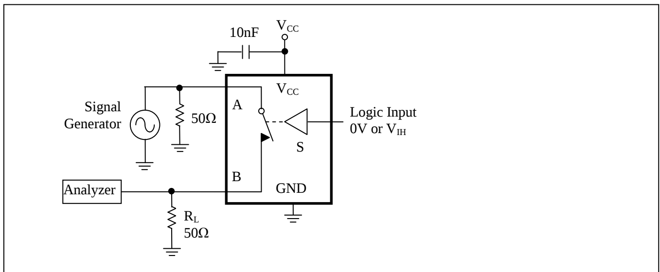
Figure 3. Off Isolation
