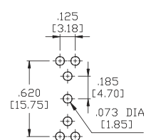
P.C.MOUNTING
