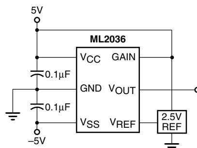
Figure 8. Sine Wave Generator with \pm 2.5V_{p-p} .
