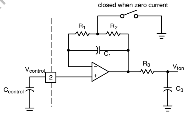
Figure 29. V_{control} Processing Circuit
