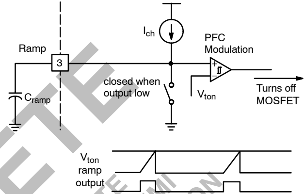
Figure 28. PFC Modulation Circuit and Timing Diagram
