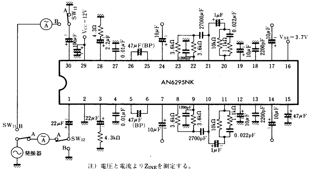
Test Circuit 9 ( Z_{INE} )
