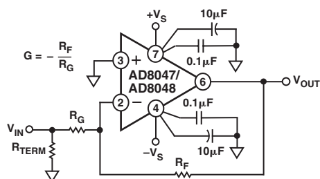
Figure 4. Inverting Operation
