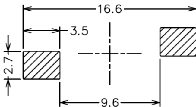
Soldering patterns
