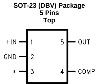
Pin Functions
