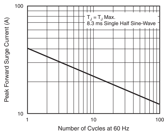
Fig. 6 - Max. Non-Repetitive Forward Surge Current Uni-Directional Only
