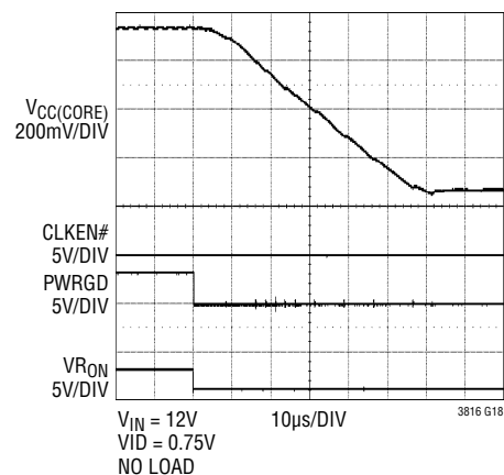
V_{RON} Shutdown
