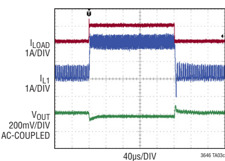
50mA to 1A Load Step
