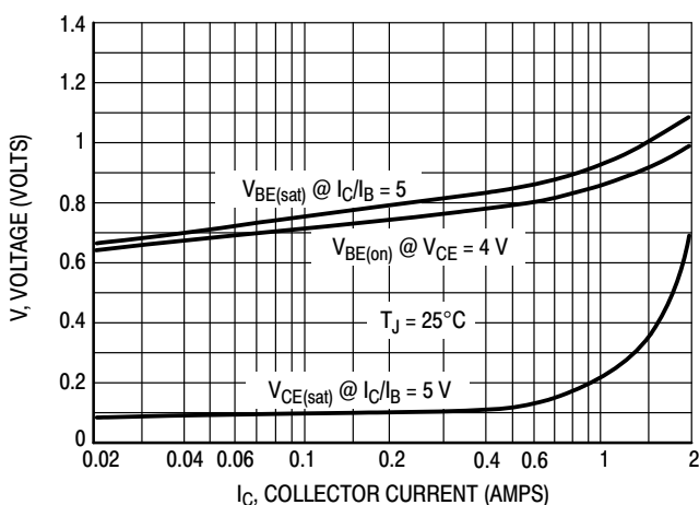
Figure 2. "On" Voltages
