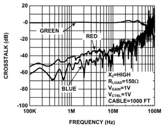
FIGURE 18. GREEN CROSSTALK
