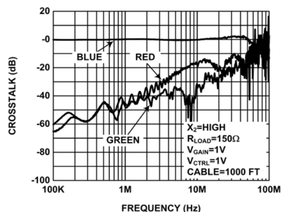
FIGURE 16. BLUE CROSSTALK
