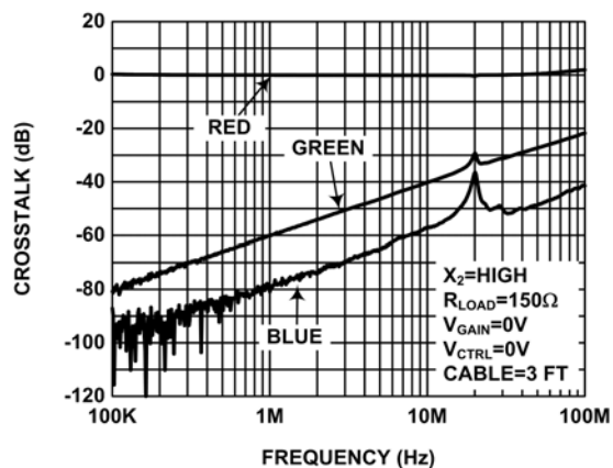
FIGURE 19. RED CROSSTALK
