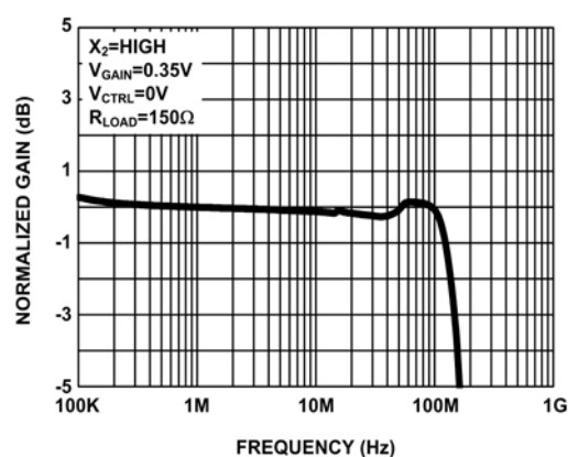
FIGURE 2. GAIN vs FREQUENCY ALL CHANNELS
