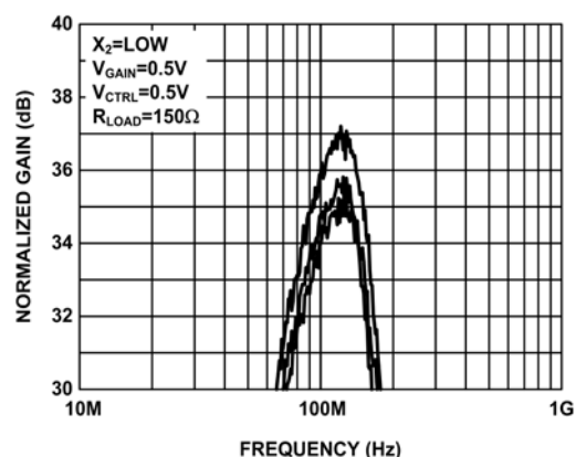
FIGURE 6. CHANNEL MISMATCH
