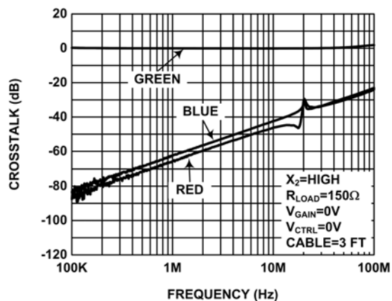
FIGURE 17. GREEN CROSSTALK
