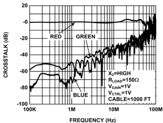
FIGURE 20. RED CROSSTALK
