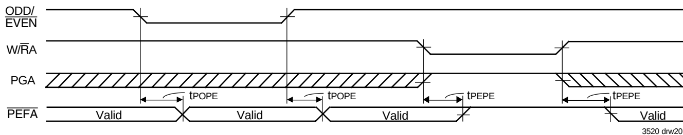
Figure 20. ODD/EVEN, W/\overline{RA} and PGA to \overline{PEFA} Timing
