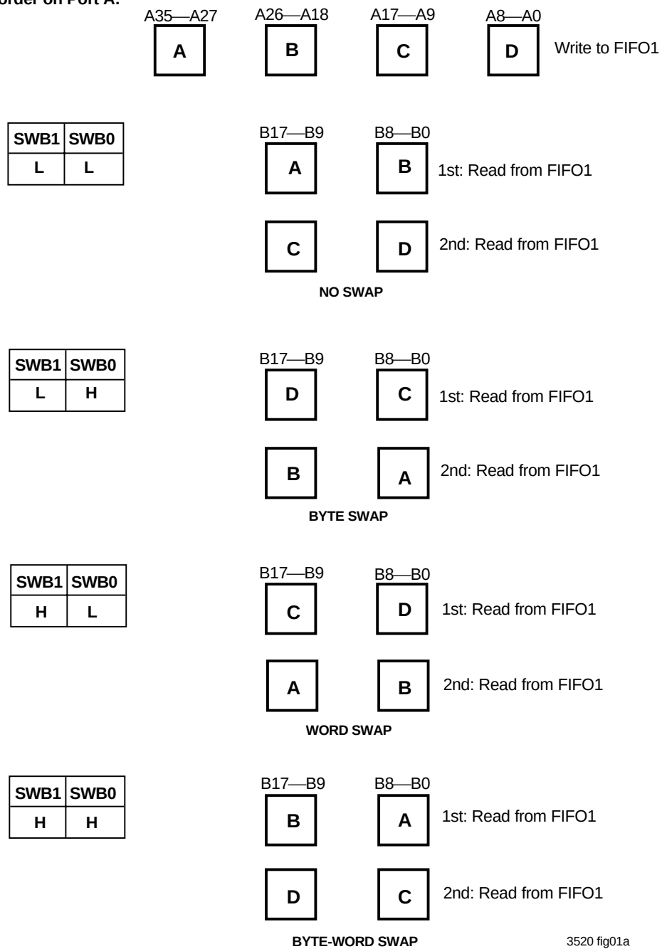
Figure 3. Port B Byte Swapping (Word Size Example)
