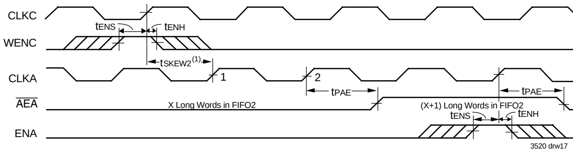
Figure 16. Timing for \overline{AEB} when FIFO1 is Almost-Empty
