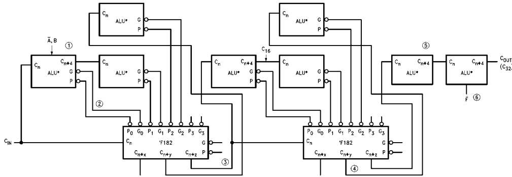
FIGURE 1. 32-Bit ALU with Riddled Carry between 16-Bit Lookahead ALUs
