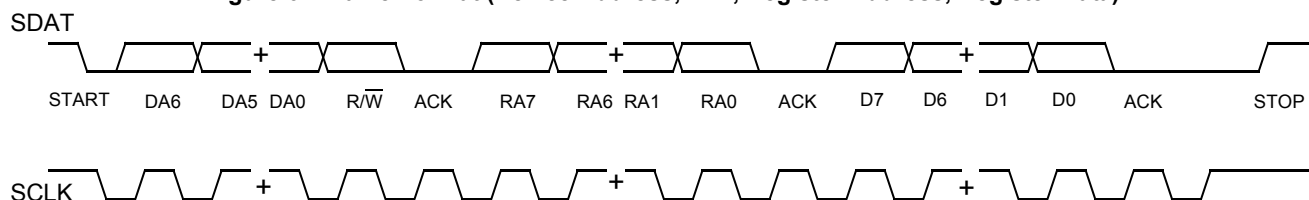
Figure 6. Frame Format (Device Address, \overline{R/\overline{W}} , Register Address, Register Data)
