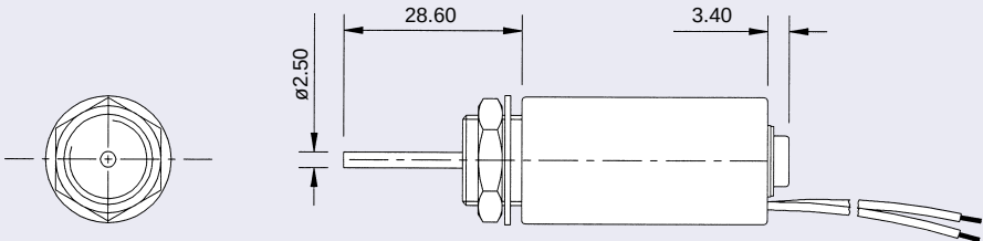
Pull type - shown energised
