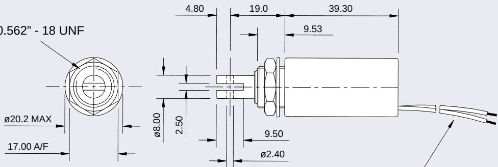
Pull type - shown energised
