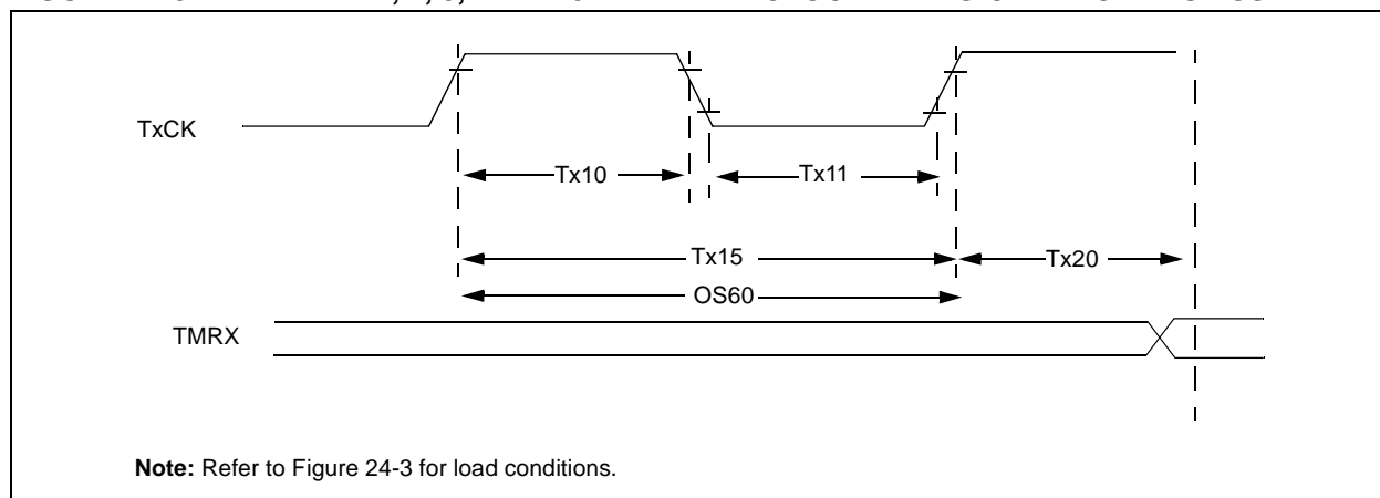
FIGURE 24-8: TIMER 1, 2, 3, 4 AND 5 EXTERNAL CLOCK TIMING CHARACTERISTICS
