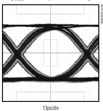
ELECTRICAL EYE DIAGRAM ( I_{MOD} = 100mA , 2^{13} - 1 + 80CID )
