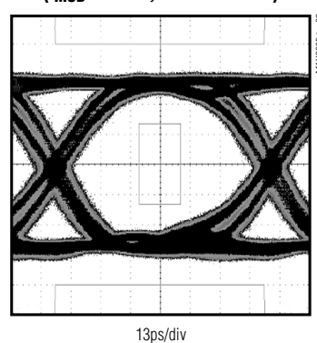
ELECTRICAL EYE DIAGRAM ( I_{MOD} = 20mA , 2^{13} - 1 + 80CID )
