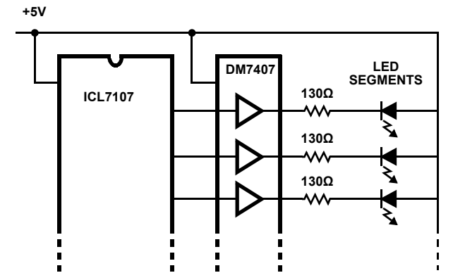
FIGURE 22. DISPLAY BUFFERING FOR INCREASED DRIVE CURRENT
