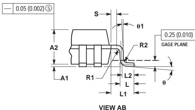
VIEW AB
