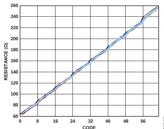
Figure 101. Typical CML Resistor Value vs. Register Code
