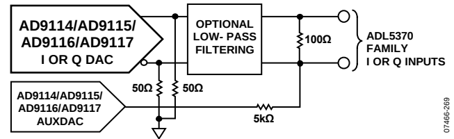
Figure 108. Typical Use of Auxiliary DACs When DC Coupling to Quadrature Modulator ADL537x Family
