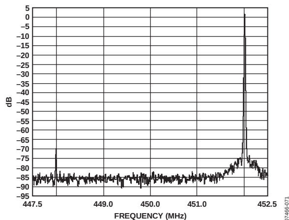
Figure 110. AD9114/AD9115/AD9116/AD9117 and ADL5370 with a Single-Tone Signal at 450 MHz, Gain and LO Compensation Optimized
