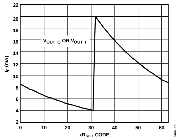
Figure 98. Effect of xR_{SET} Code
