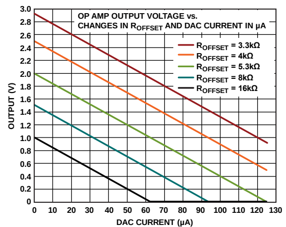
Figure 106. AUXDAC Op Amp Output vs. Current, AVDD = 3.3 V No Load, AUXDAC 0x1FF to 0x000
