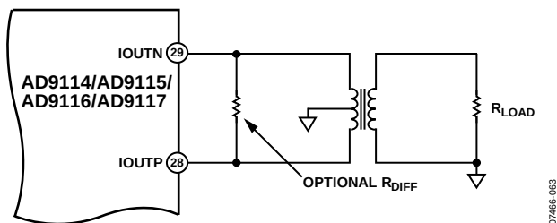
Figure 102. Differential Output Using a Transformer
