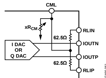
Figure 100. Simplified Internal Load Options
