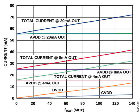
Figure 83. AD9114/AD9115/AD9116/AD9117 Supply Current vs. f_{DAC} , 3.3 V
