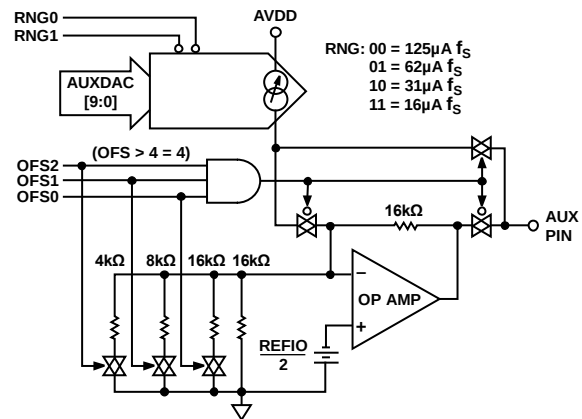
Figure 105. AUXDAC Simplified Circuit Diagram
