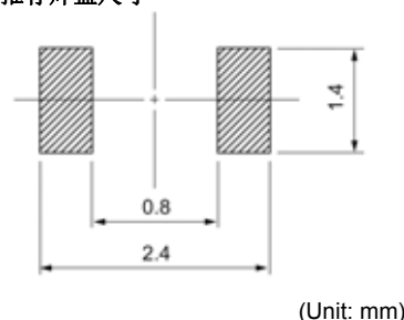
Recommended patterns 推荐焊盘尺寸
