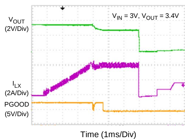
Overload Protection
