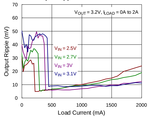
Output Ripple vs. Load Current
