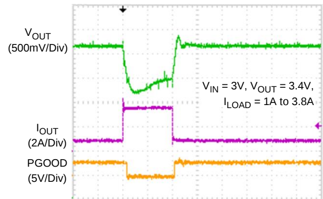
Transient Overload
