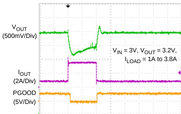
Transient Overload
