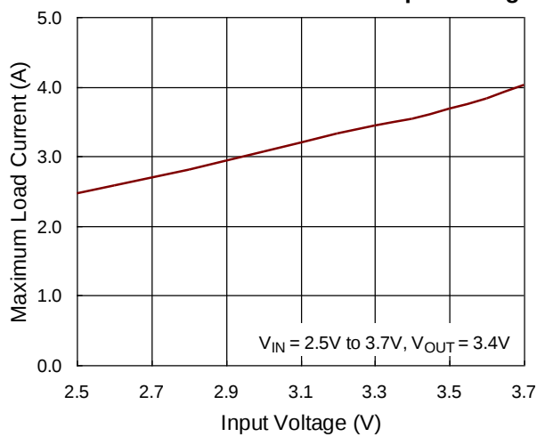
Maximum Load Current vs. Input Voltage
