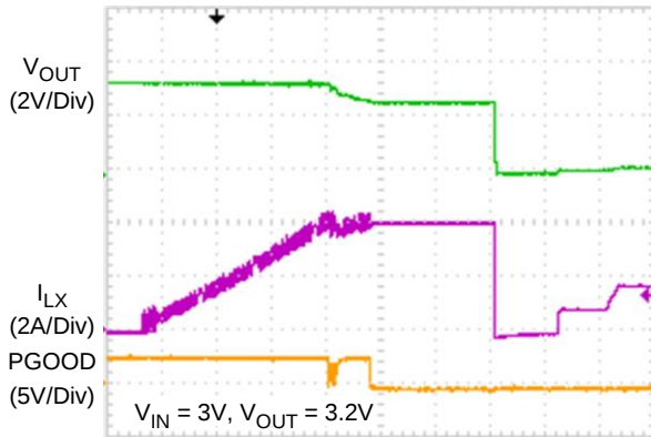
Overload Protection
