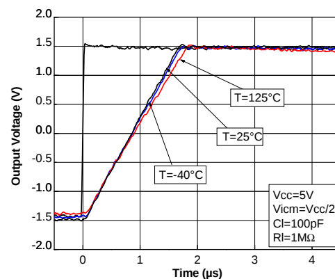
Figure 15. Positive slew rate at V_{CC} = 5\text{ V} with C_L = 100\text{ pF}
