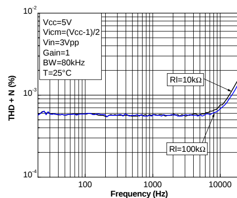
Figure 19. Distortion + noise vs. frequency
