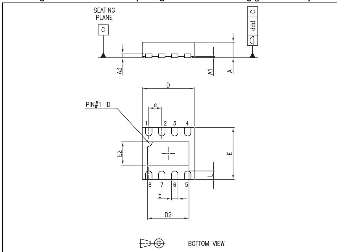
Figure 28. DFN8 2 x 2 mm package mechanical drawing (pitch 0.5 mm)
