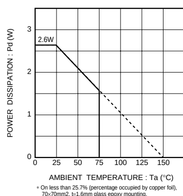
Fig.4 Power dissipation
