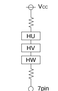
〈 Series connection 〉
