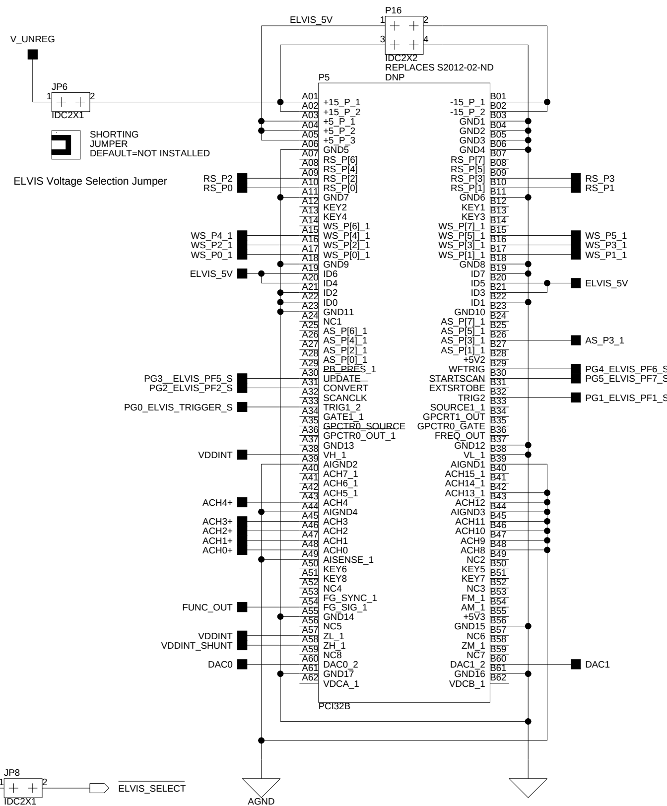
ELVIS CONNECTOR
